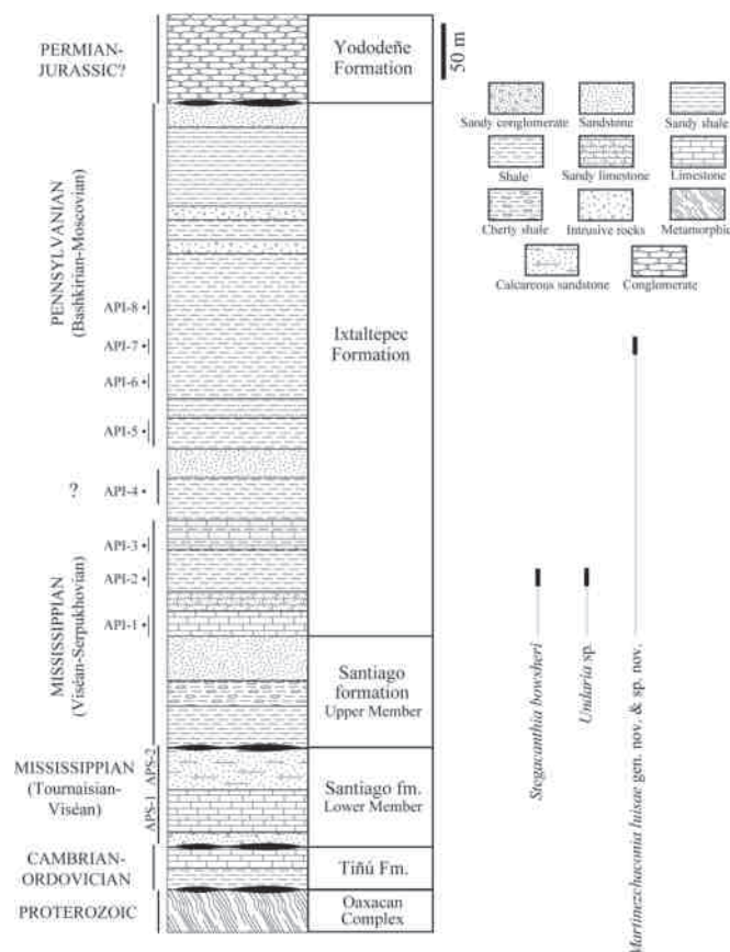
Figure 2. Stratigraphic column of the Santiago Ixtaltepec region. It shows the relationship between the different units that have been recognized and the location of the stratigraphic units in which brachiopods described were collected.
